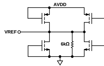
Figure 62. Equivalent VREF Circuit
