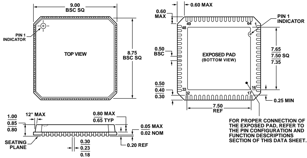
COMPLIANT TO JEDEC STANDARDS MO-220-VMM4-4 Figure 85. 64-Lead Lead Frame Chip Scale Package [LFCSP_VQ] 9 mm × 9 mm Body, Very Thin Quad (CP-64-6) Dimensions shown in millimeters
