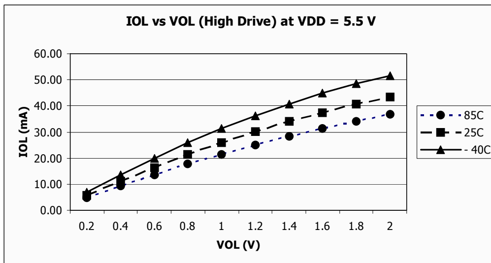
Figure 24. Typical I_{OL} vs. V_{OL} V_{DD} = 5.5 V (High Drive)
