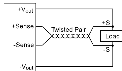
Fig.72 Sense connections
