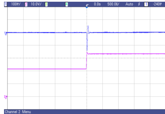
Fig.37 AVO505-48S2V5 typical transient response to step increase in load from 50% to 75% of full load, room temperature, 48Vdc input ( \Delta I_o/\Delta t = 1A/1\mu s )
