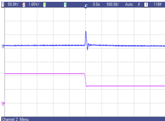
Fig.22 AVO50-48S1V2 typical transient response to step decrease in load from 50% to 25% of full load, room temperature, 48Vdc input ( \Delta I_o/\Delta t = 0.1A/1\mu s )
