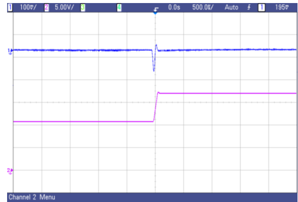
Fig. 43 AVO50-48S05 typical transient response to step increase in load from 50% to 75% of full load, room temperature, 48Vdc input ( \Delta I_o/\Delta t = 0.1A/1\mu s )
