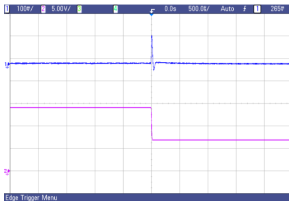
Fig.44 AVO50-48S05 typical transient response to step decrease in load from 50% to 25% of full load, room temperature, 48Vdc input ( \Delta I_o/\Delta t = 1A/1\mu s )
