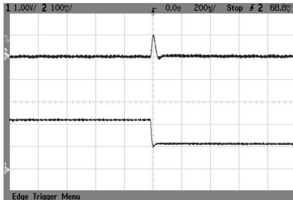
Fig.28 AVO50-48S1V5 typical transient response to step decrease in load from 50% to 25% of full load, room temperature, 48Vdc input ( \Delta I_o/\Delta t = 1A/1\mu s )
