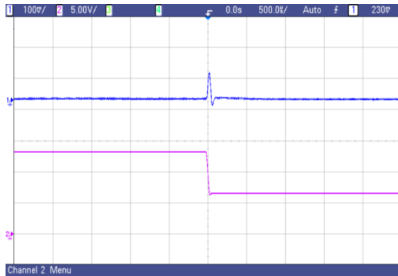
Fig.42 AVO50-48S05 typical transient response to step decrease in load from 50% to 25% of full load, room temperature, 48Vdc input ( \Delta I_o/\Delta t = 0.1A/1\mu s )
