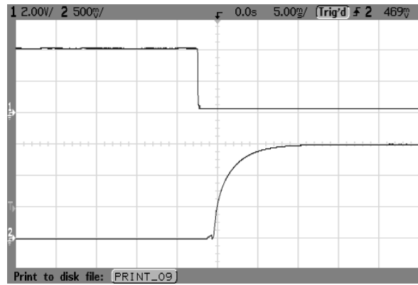
Fig.60 AVO50-48S1V5 typical start-up from CNT on
