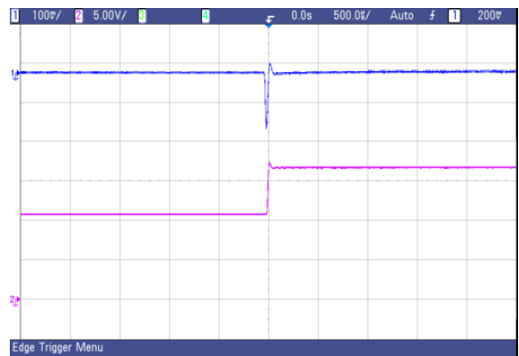
Fig.45 AVO50-48S05 typical transient response to step increase in load from 50% to 75% of full load, room temperature, 48Vdc input ( \Delta I_o/\Delta t = 1A/1\mu s )
