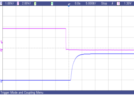
Fig.64 AVO50-48S2V5 typical start-up from CNT on
