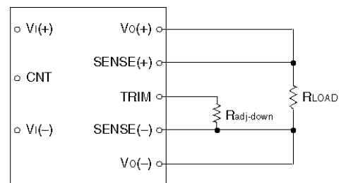
Fig.74 Trim down circuit
