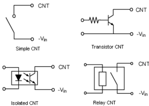
Fig.71 CNT circuits
