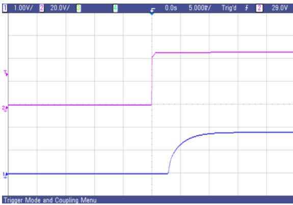
Fig.61 AVO50-48S1V8 typical start-up from power on
