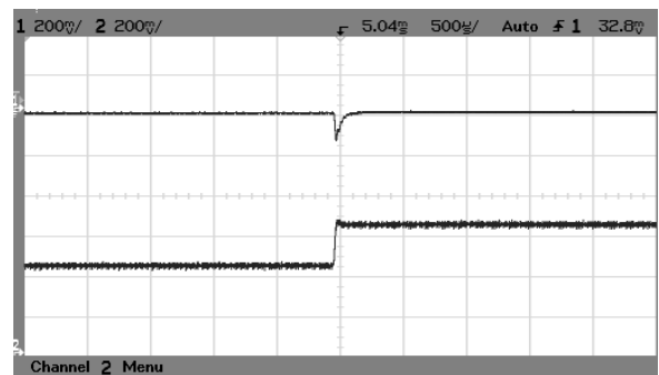
Fig. 47 AVO50-48S12 typical transient response to step increase in load from 50% to 75% of full load, room temperature, 48Vdc input ( \Delta I_o/\Delta t = 0.1A/1\mu s )
