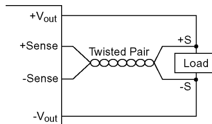
Fig.72 Sense connections
