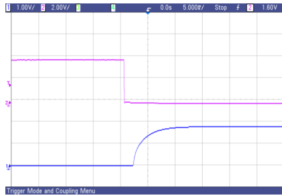
Fig.62 AVO50-48S1V8 typical start-up from CNT on
