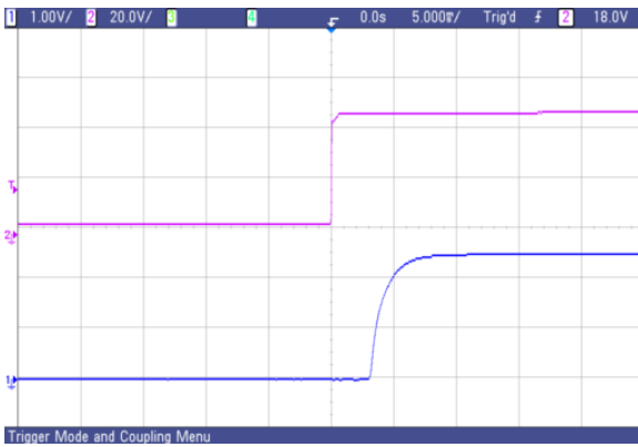
Fig.63 AVO50-48S2V5 typical start-up from power on
