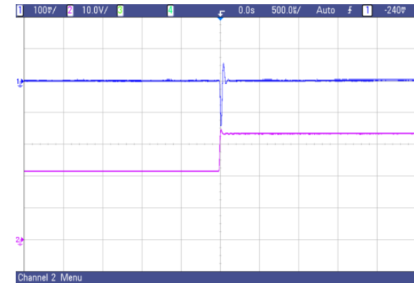
Fig.37 AVO50-48S2V5 typical transient response to step increase in load from 50% to 75% of full load, room temperature, 48Vdc input ( \Delta I_o/\Delta t = 1A/1\mu s )
