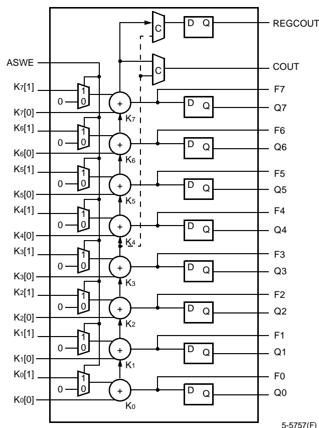
Figure 8. Multiplier Submode
