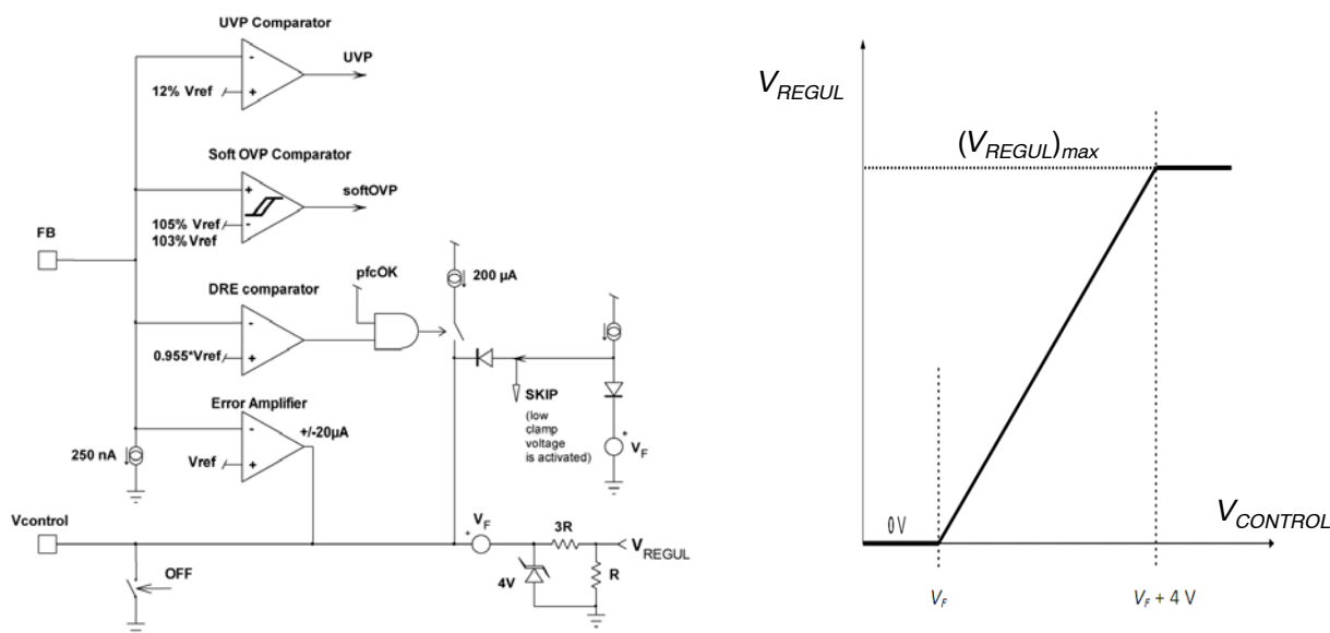
Figure 67. a) Regulation Block Figure (left), b) Correspondence between V_{\text{CONTROL}} and V_{\text{REGIII}} (right)
