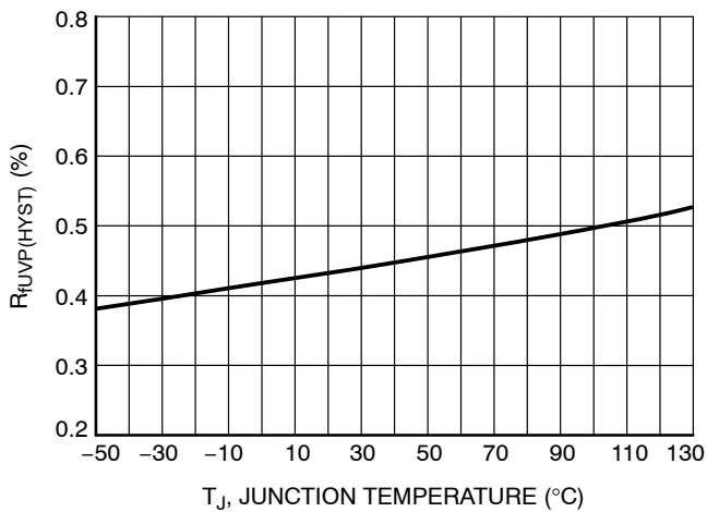
Figure 49. Ratio (UVP Hysteresis) over V REF vs. Temperature
