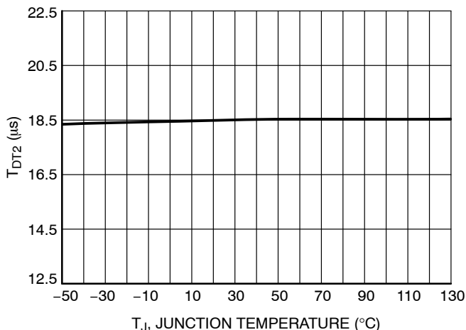
Figure 11. Dead-Time, V FFcontrol = 1.75 V vs. Temperature
