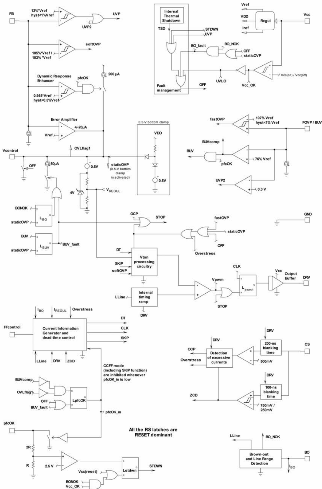
Figure 2. Block Diagram
