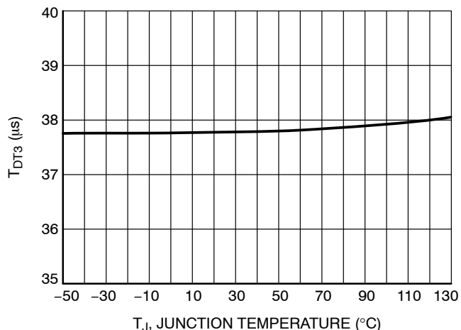
Figure 12. Dead-Time, V FFcontrol = 1.00 V vs. Temperature
