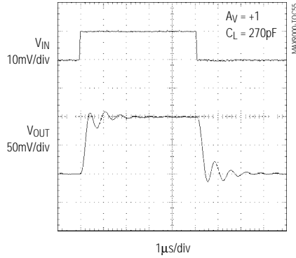
MAX9003/MAX9004/MAX9005 OP-AMP SMALL-SIGNAL TRANSIENT RESPONSE WITH C LOAD
