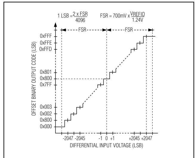
Figure 7. Binary Transfer Function ( T/B = 1 )
