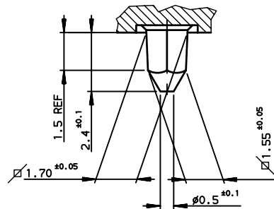
DETAIL OF LOCATING PEGS (2x) SCALE B/1
