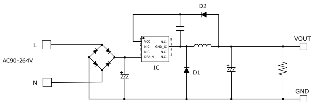
Figure 4. BM2P249TF-EVK-001 Application Circuit
