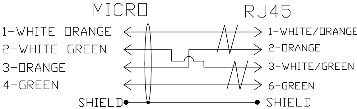
WIRE DIAGRAM
