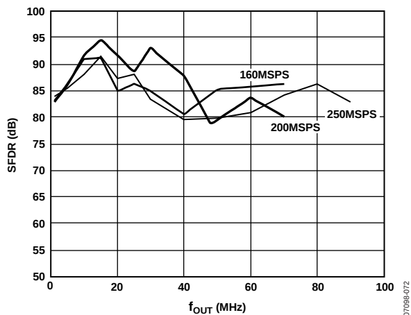
Figure 13. AD9787 In-Band SFDR vs. f_{OUT} , 2× Interpolation
