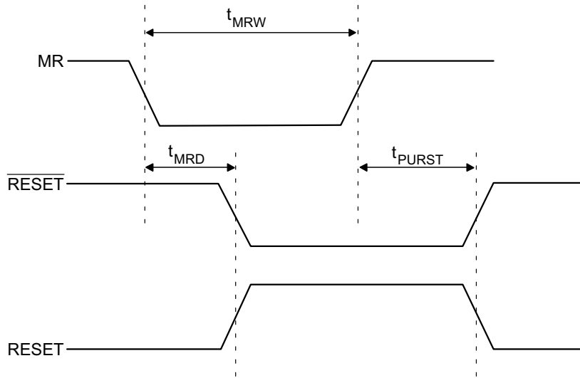
Figure 2. \overline{\text{MR}} Operation and Timing
