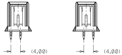
SECTION: Y-Y SECTION: W-W
