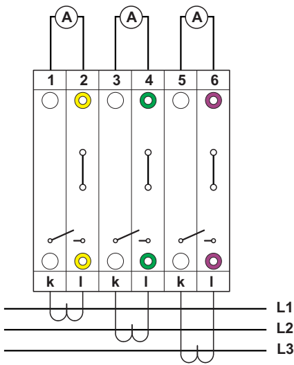
Connection diagram
