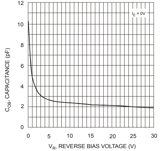
Fig. 4 Output Capacitance
