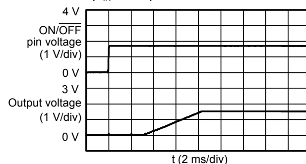
S-8533A33AFT ( V_{IN} : 9.0\text{ V} )
