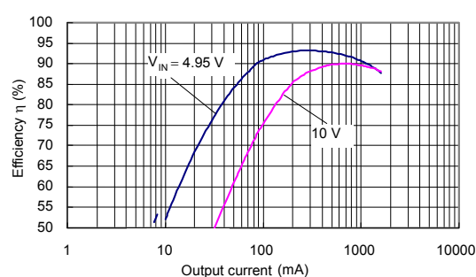
(24) S-8533A50AFT (Si3454DV/Si3455DV)
