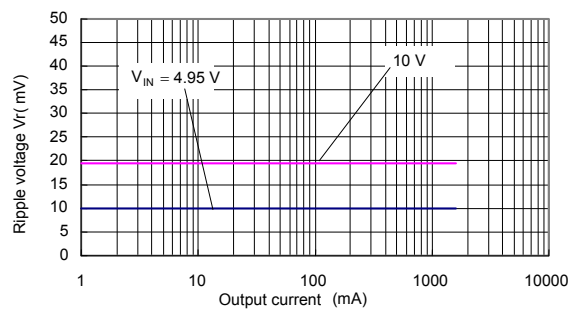
(34) S-8533A50AFT (Si3454DV/Si3455DV)
