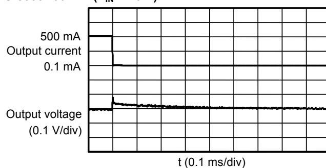
S-8533A50AFT ( V_{IN} : 7.5 \text{ V} )
