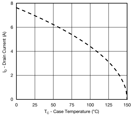
Current Derating*
