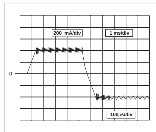
Figure 4. Motor current ( I_M ), Vertical : 200 mA/div, Horizontal: 1 ms/div, expanded part 100 µs/div.
