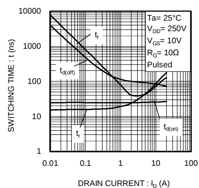
Fig.14 Switching Characteristics
