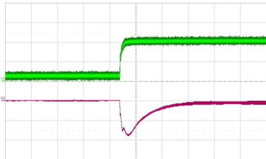
Figure 15. Load transient V 1 , 5 to 40 A (500 μs/div) CH2: V 1 (200 mV/div) CH4: I 1 (20 A/div)
