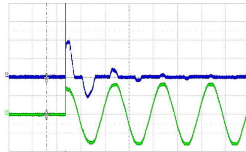
Figure 5. Inrush current, V_{in} = 230Vac, 90^\circ CH4: V_{in} (200V/div), CH2: I_{in} (20 A/div)
