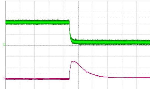
Figure 16. Load transient V 1 , 40 to 5 A (500 μs/div) CH2: V 1 (200 mV/div) CH4: I 1 (20 A/div)
