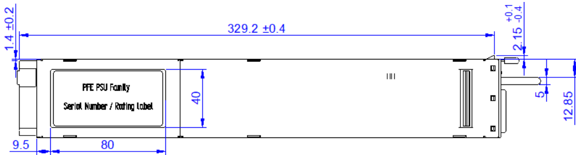
Figure 44. Top View
