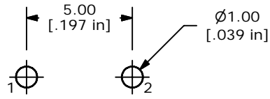
PC MOUNTING
