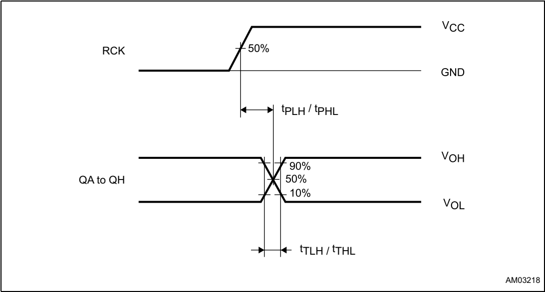
Figure 8. Waveform 2: RCK to QN propagation delay times ( f = 1\text{ MHz} ; 50 % duty cycle)
