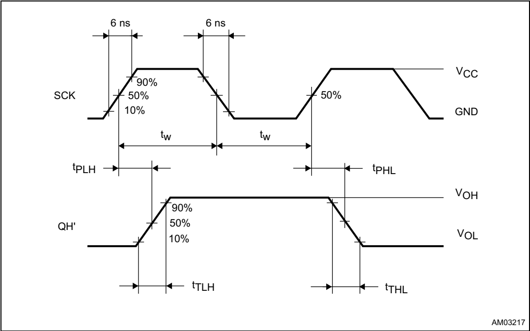
Figure 7. Waveform 1: SCK to QH' propagation delay times, SCK minimum pulse width ( f = 1\text{ MHz} ; 50 % duty cycle)
