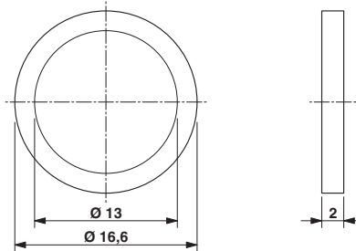
Dimensioned drawing
