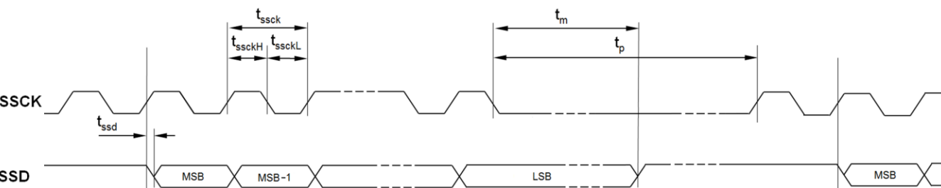
Figure 15: SSI Timing
