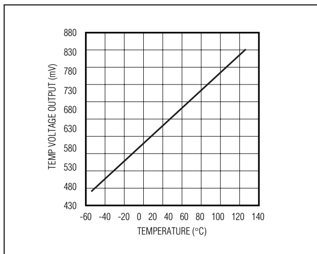
Figure 2. MAX675 Temperature Voltage Output vs. Temperature
