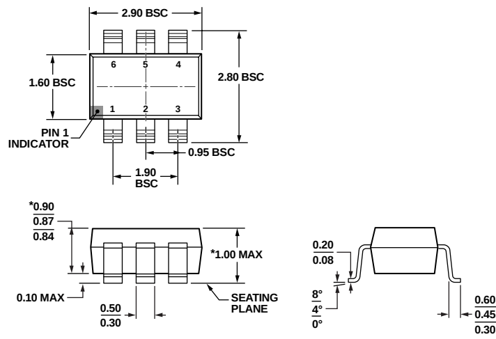
*COMPLIANT TO JEDEC STANDARDS MO-193-AA WITH THE EXCEPTION OF PACKAGE HEIGHT AND THICKNESS. Figure 59. 6-Lead Thin Small Outline Transistor Package [TSOT] (UJ-6) Dimensions shown in millimeters
