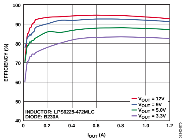
Figure 4. Efficiency Curve, V_{IN} = 18\text{ V} , f_{SW} = 1.4\text{ MHz}
