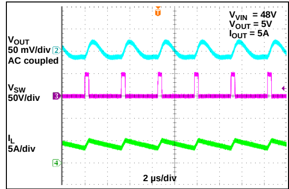
FIGURE 2-57: Switching Waveform at Full Load.
