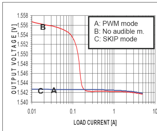
Figure 13. 1.5 V voltage regulation vs load current
