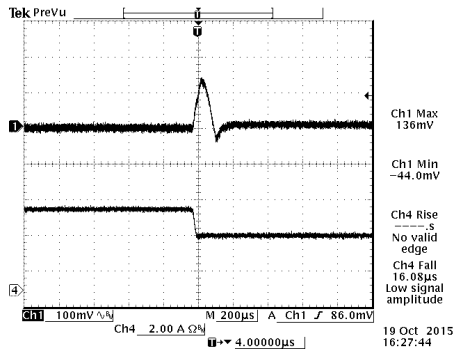
Figure 7. 75%-50% Load Transients at Vin=110V@Ta=25°C
