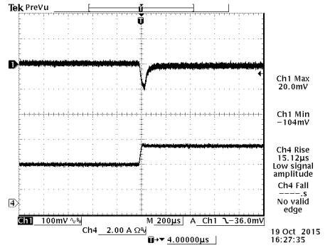
Figure 5. 50%-75% Load Transients at Vin=110V@Ta=25°C
