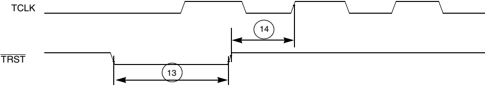
Figure 13. \overline{\text{TRST}} Timing
