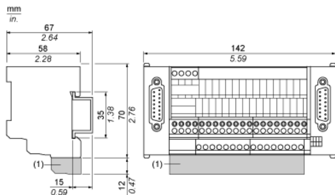
(1) ABE7BV10 / ABE7BV20
