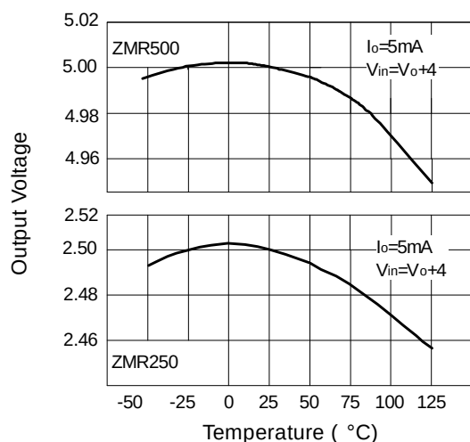
Output Voltage Temperature
