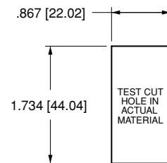
MOUNTING HOLE
