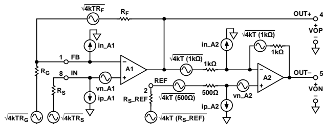
Figure 52. Noise Sources
