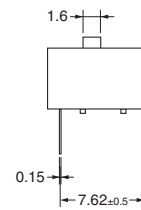
Raised Actuator
