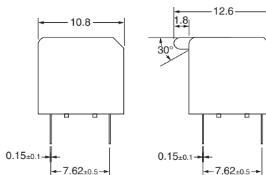
Side Actuator (short-lever)
