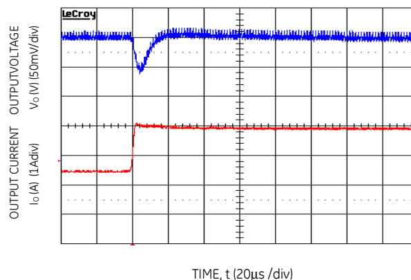
Figure 28. Transient Response to Dynamic Load Change from 50% to 100% at 12V in , C out -2x47μF, C Tune -2200pF & R Tune -261
