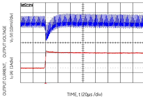
Figure 10. Transient Response to Dynamic Load Change from 50% to 100% at 12V in , C_{out}=1\times 47\mu\text{F}+1\times 330\mu\text{F} , C_{TUNE}=10\text{nF} & RTune-261
