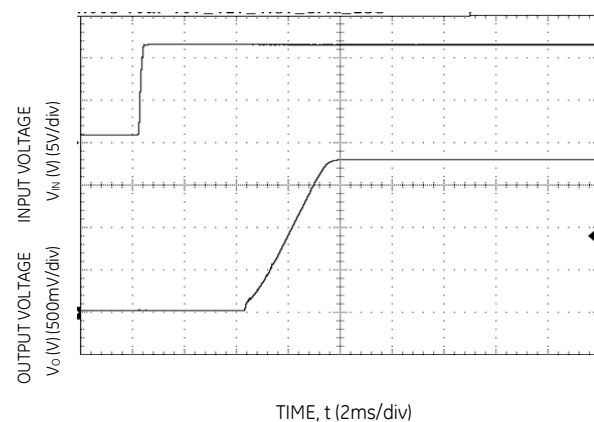
Figure 18. Typical Start-up Using Input Voltage ( V_{in}=12\text{V} , I_o=I_{o,max} ).
