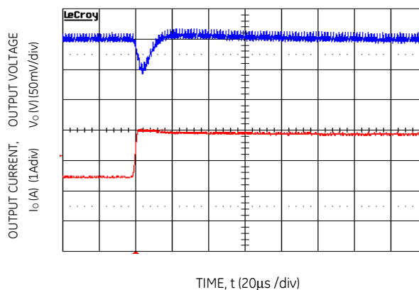
Figure 22. Transient Response to Dynamic Load Change from 50% to 100% at 12V in , C out =2x47μF, C Tune =2700pF & RTune-261
