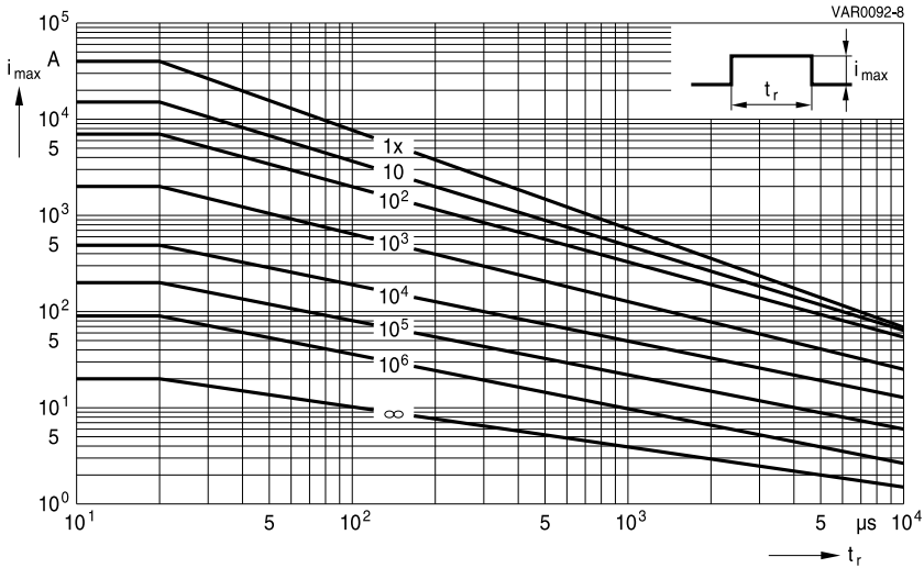
SIOV-B40K230 ... K460
