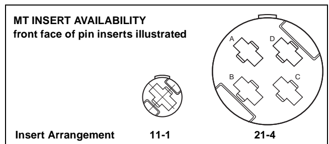
Tri-Start (MIL-DTL-38999, Series III) Connectors with MT Ferrule Inserts
