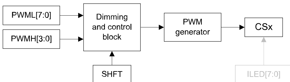
Figure 6. Digital dimming
