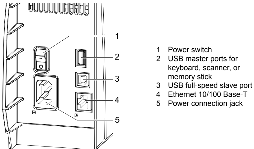
Fig. 6 Connections
