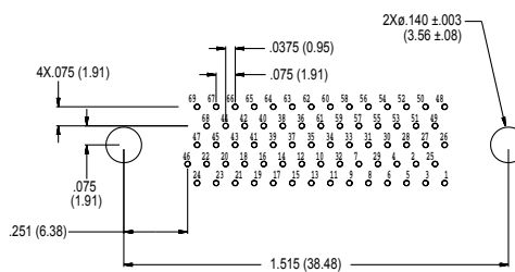
69 PIN MWDM-69PCBS
