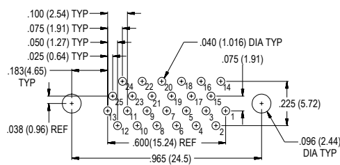
25 PIN MWDM-25PCBS
