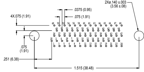
69 Socket MWDM-69SCBS
