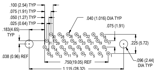
31 PIN MWDM-31PCBS
