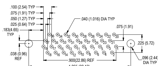
37 PIN MWDM-37PCBS
